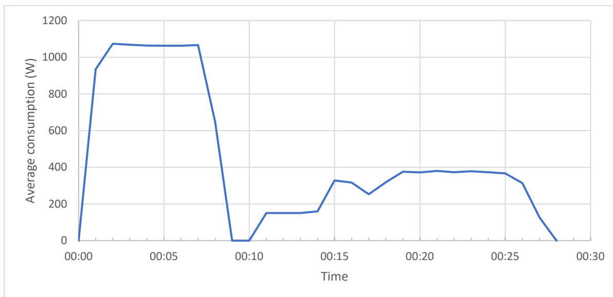
Figure 2.101 Plot of average consumption per minute measured with a Shelly Plus smart plug for the SQ Professional single electric hot plate hob starting on setting 5 and turned down to 3
