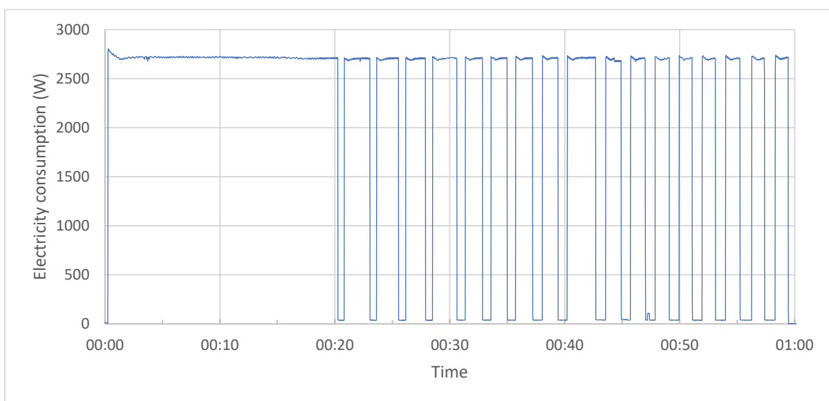
Figure 2.48 Plot of apparent power consumption measured every second with a Tinytag View 2 for the fan oven for a Rangemaster Professional Plus Range Cooker at 200°C
