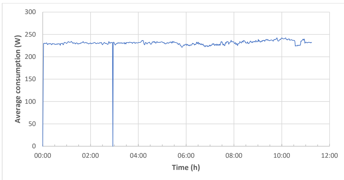
Figure 2.25 Average electricity consumption for an Argos 220W heated ailer with wings
