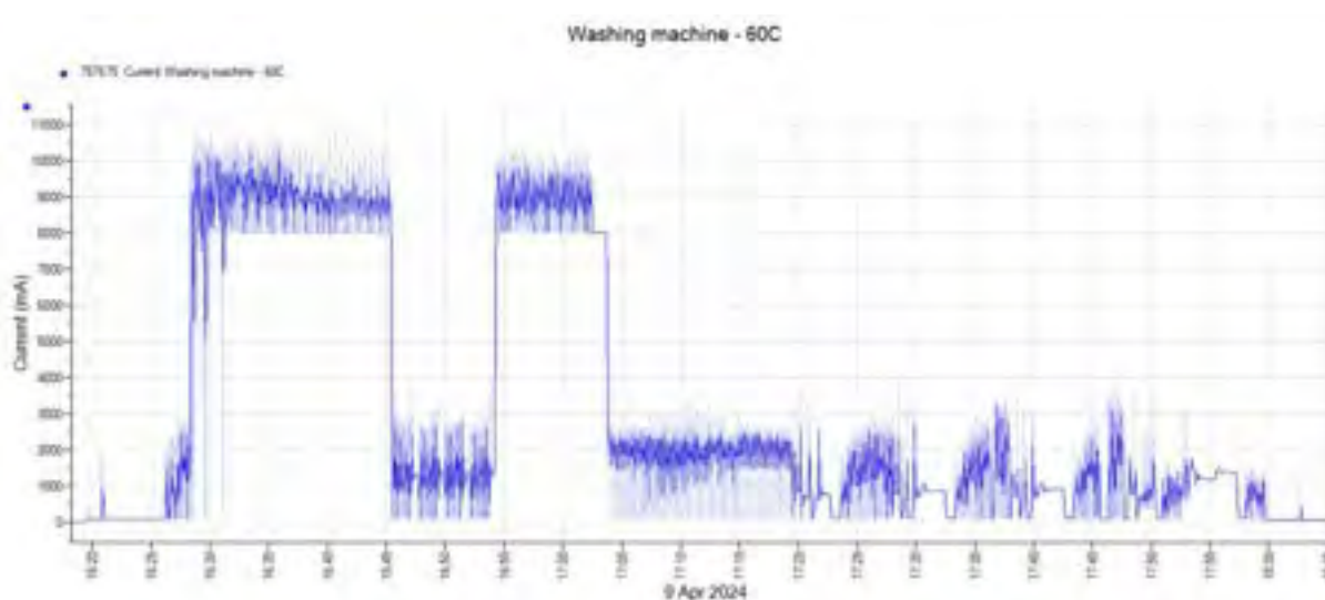
Figure 3.4 Plot of consumption for a Hotpoint WMTL80 washing machine recorded using a Tinytag View 2 data logger at 1 second intervals for a 60°C washing cycle
