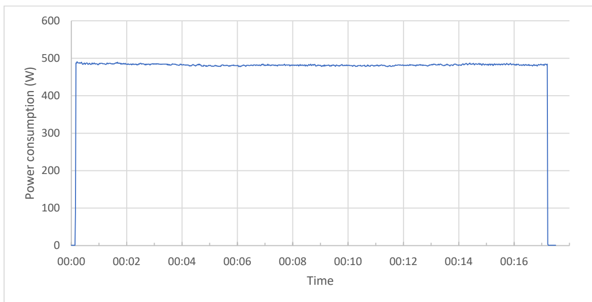
Figure 2.109 Plot of apparent power consumption measured every second with a Tinytag View 2 for the Salter EK2726 steamer
