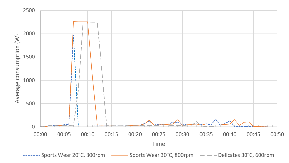
Figure 2.14 Plot of average consumption per minute measured with the Shelly Plus smart plug for the Bosch WGG04409GB washing machine on low temperature, low spin cycles
