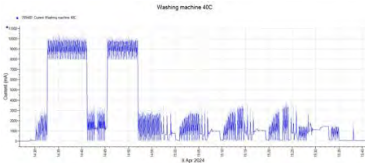
Figure 3.3 Plot of consumption for a Hotpoint WMTL80 washing machine recorded using a Tinytag View 2 data logger at 1 second intervals for a 40°C washing cycle
