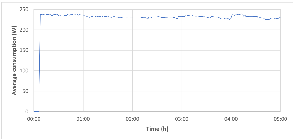
Figure 2.24 Average electricity consumption for a Dunelm 220W heated ailer with wings
