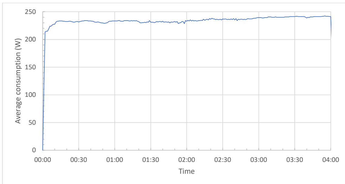
Figure 2.34 Plot of average consumption per minute measured with the Shelly Plus smart plug for the MeacoDry Arete One 20L dehumidifier and air purifier operating in a damp room
