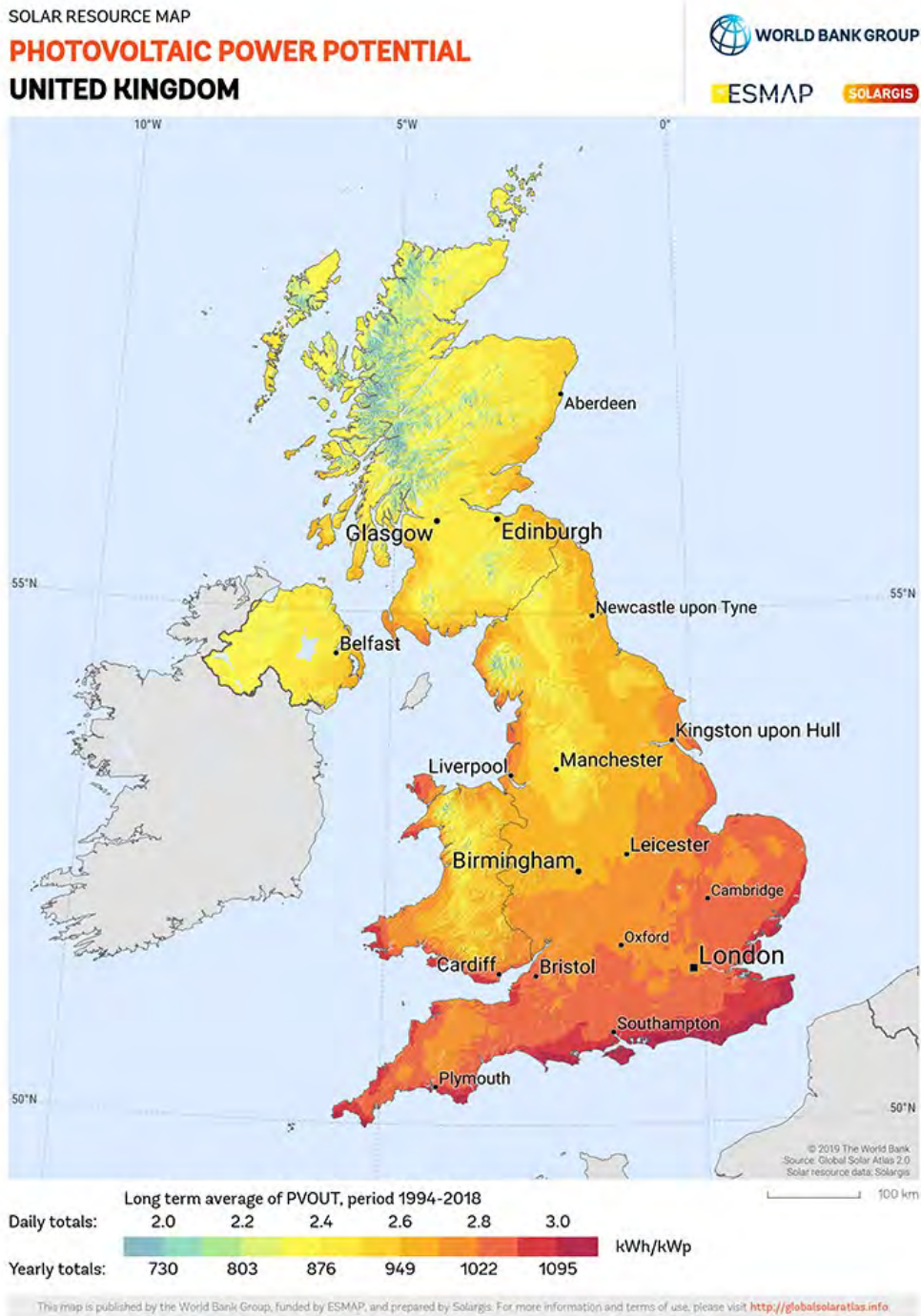
Figure 2.4 Map of Photovoltaic Power Potential (kWh/kWp) for the UK
