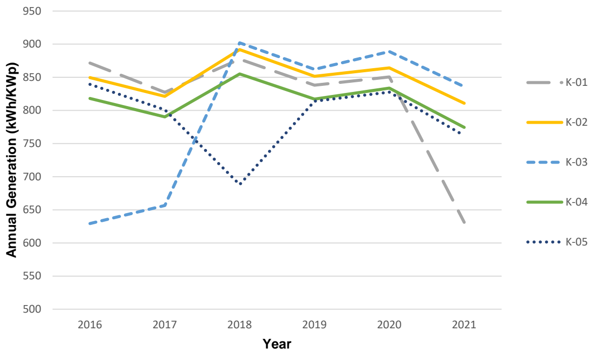
Figure 8.23 Graph of annual generation between 2016 and 2021 for properties in CCS Area K
