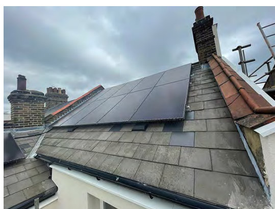
Figure 7.2 Solar PV installation in Waltham Forest
