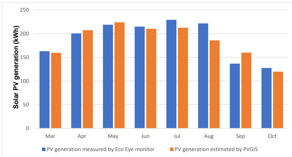
Figure 4.34 Monthly PV generation for household E-02 measured by the Eco Eye monitor and estimated using PVGIS
