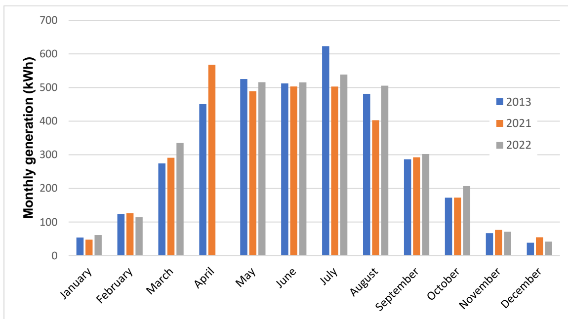
Figure 4.4 Plot of monthly solar PV generation for household W-01 based on data from the generation meter (2013) and the Wibee Box monitor (2021 and 2022)
