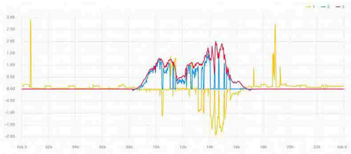
Figure 4.16 Graph from the Wibeer Nest portal showing grid import/export (in yellow), electricity consumption by the immersion heater (in blue) and PV generation (in red) for 5 Feb 23
