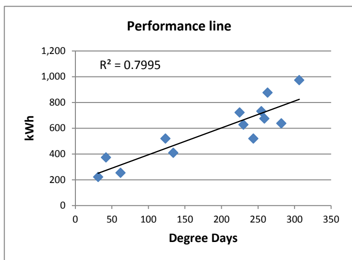
Figure 3.3a T-14 heated by storage heaters
