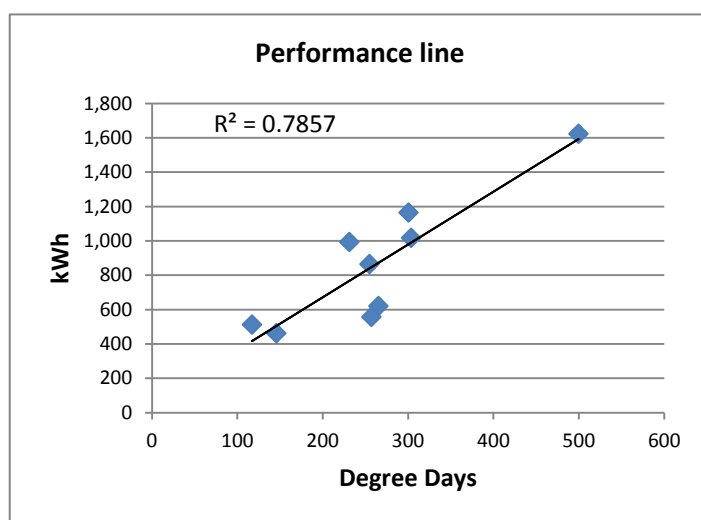
Figure 3.3b T-14 heated by hybrid system
