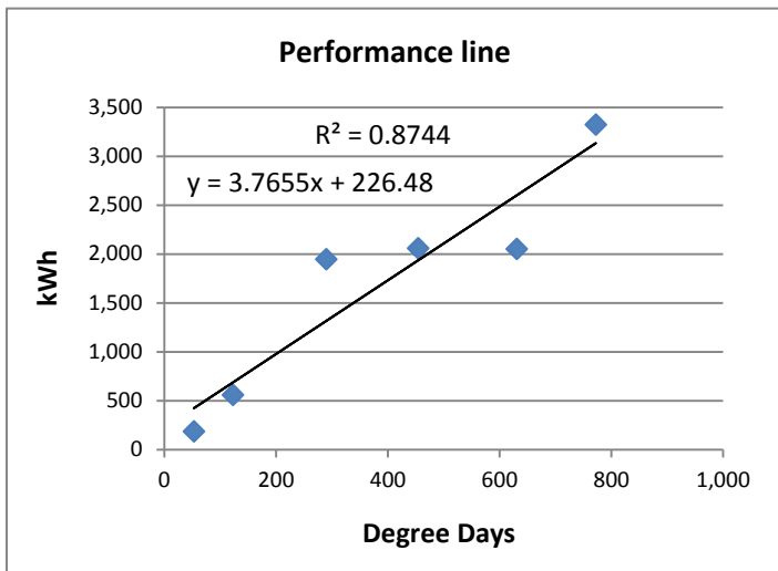
Figure 3.8a T-10 heated by storage heaters
