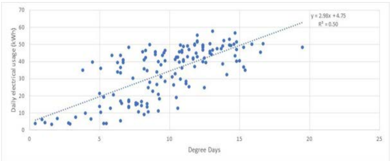
Graph 3.3.7 Property T-12 total daily electrical usage against degree days for 6 Dec 2017 to 1 May 2018
