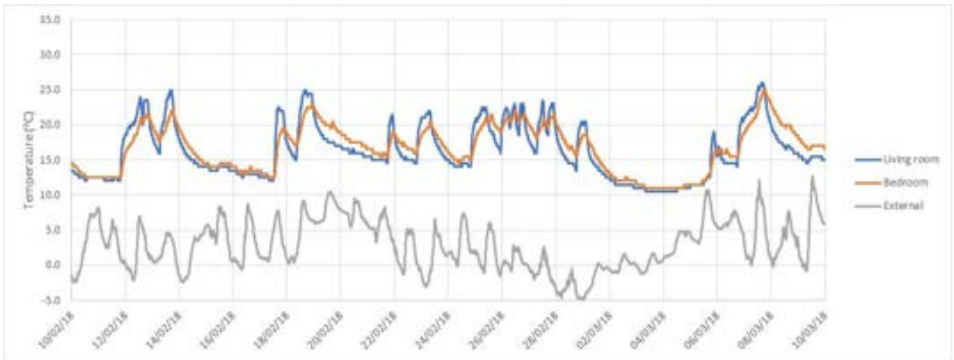
Graph 3.3.23 Property T-13 internal and external temperatures for 10 Feb to 9 Mar 2018
