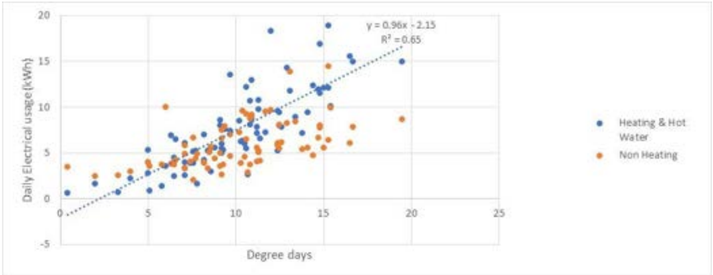
Graph 3.3.8 Property T-4 daily electrical usage against degree days for 3 Feb to 19 April 2018
