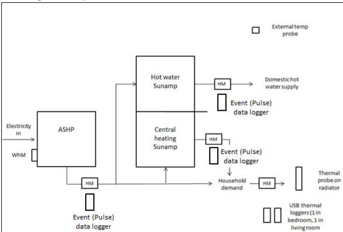
Figure 3.12 – Schematic diagrams of monitoring equipment placed in properties receiving Sunamp heat batteries,
