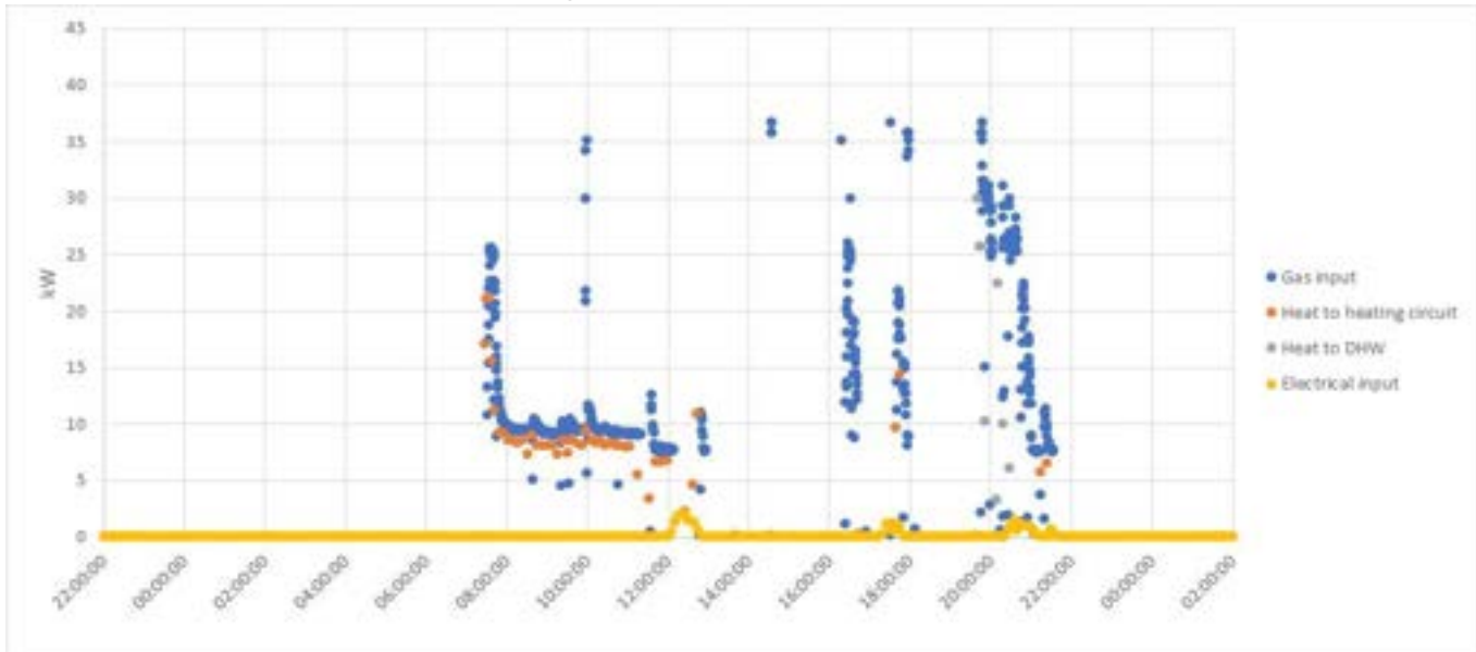
Graph 3.3.13 Property T-73 gas and electrical input to hybrid and heat output for 28 Feb 2018
