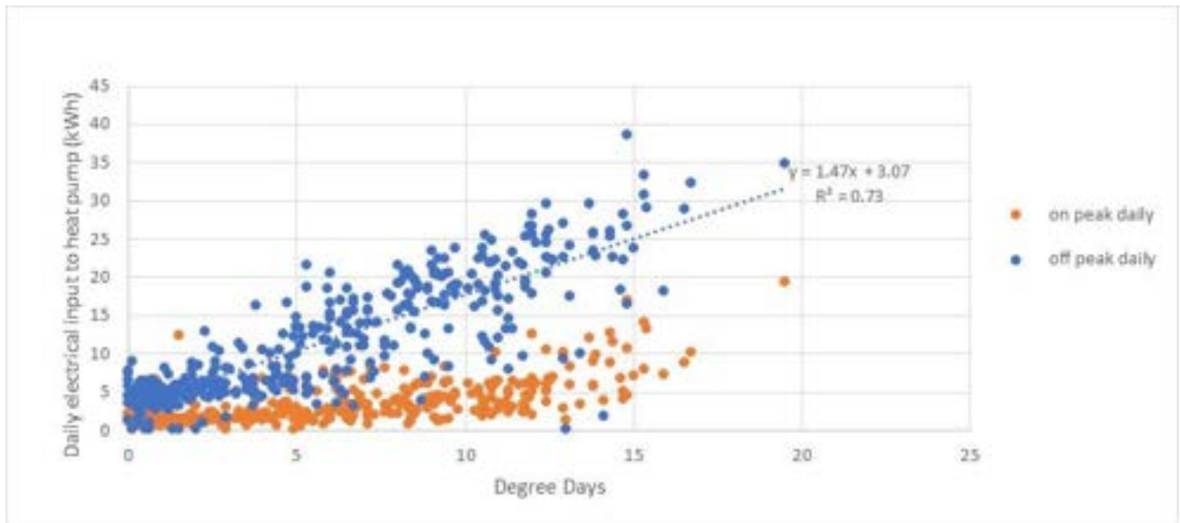
Graph 3.3.25 Property T-17 daily electrical input to heat pump against degree days - 19 Mar 2017 to 29 Apr 2018
