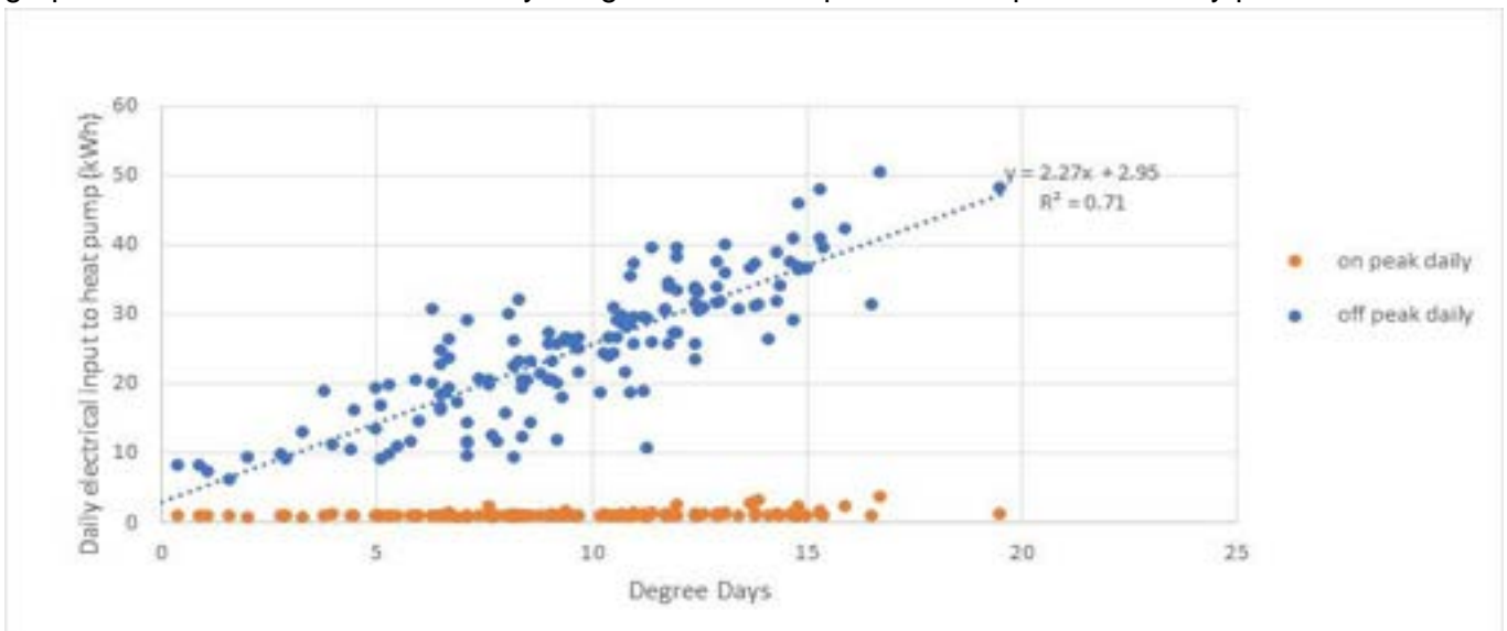
Graph 3.3.24 Property T-16 daily electrical input to heat pump against degree days - 5 Dec 2017 to 28 Apr 2018
