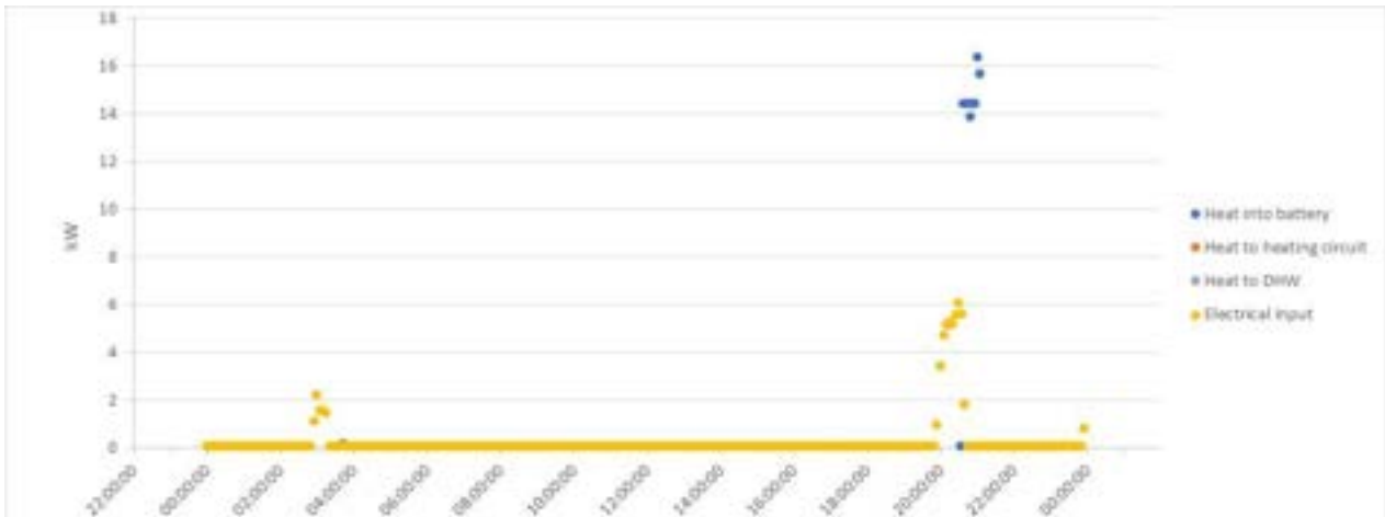
Graph 3.3.36 Property T-8 electrical input and heat output for 15 Jun 2017
