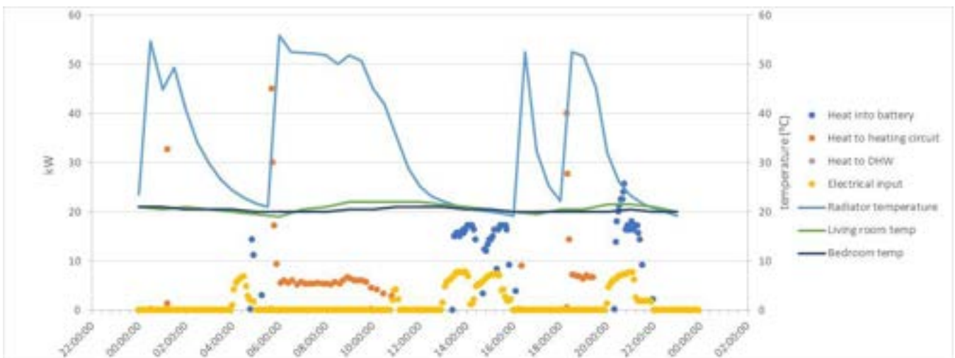
Graph 3.3.35 Property T-8 combined graph showing temperatures and energy flows for 21 Jan 2017
