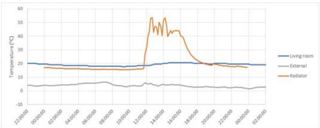
Graph 3.3.16 Property T-73 internal, external and radiator temperatures for 31 Jan 2018
