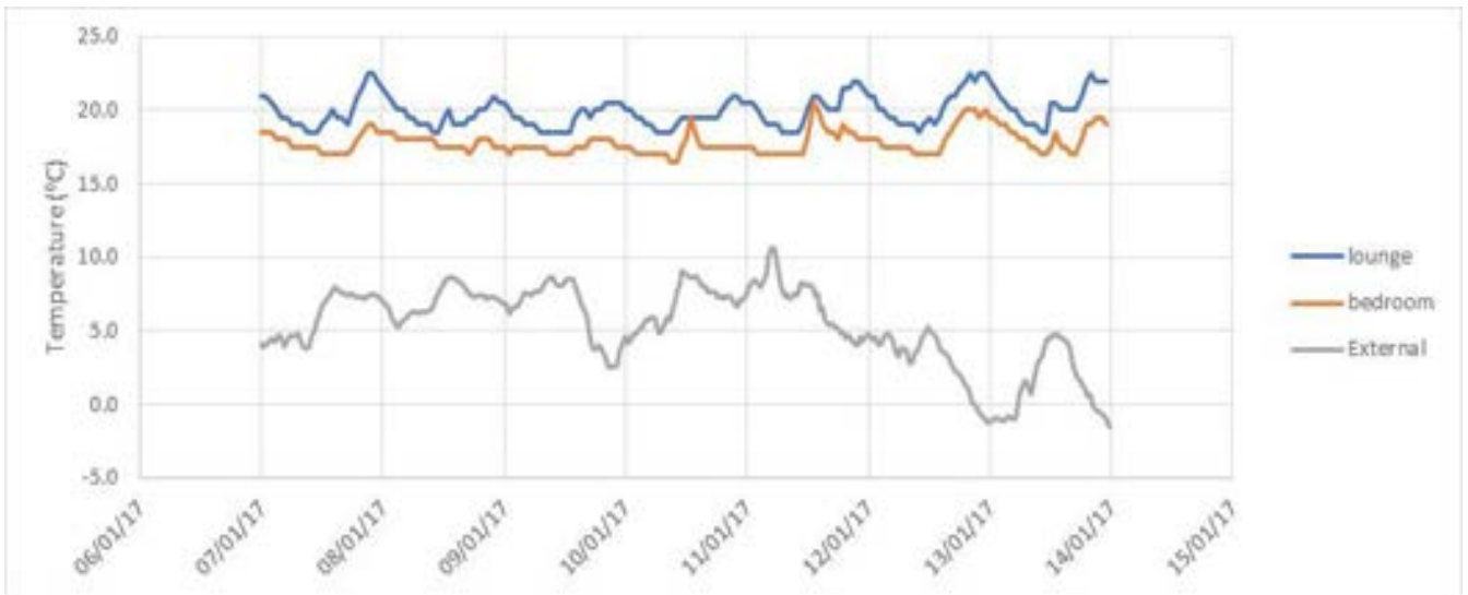
Graph 3.3.12 Property T-73 internal and external temperatures 7 to 14 Jan 2017
