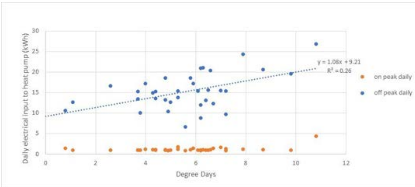
Graph 3.3.29 Property T-8 predicted daily electrical input to heat pump against degree days without timeclock error – 26 Mar to 30 Apr 2017
