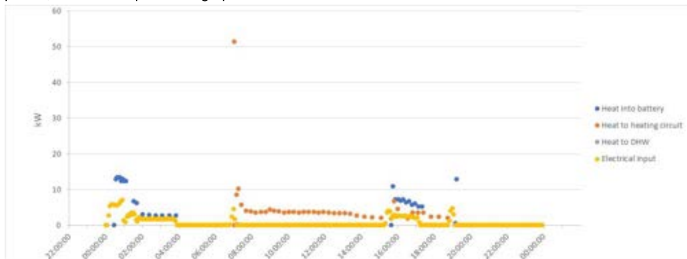
Graph 3.3.38 Property T-9 electrical input and heat output for 21 Jan 2017
