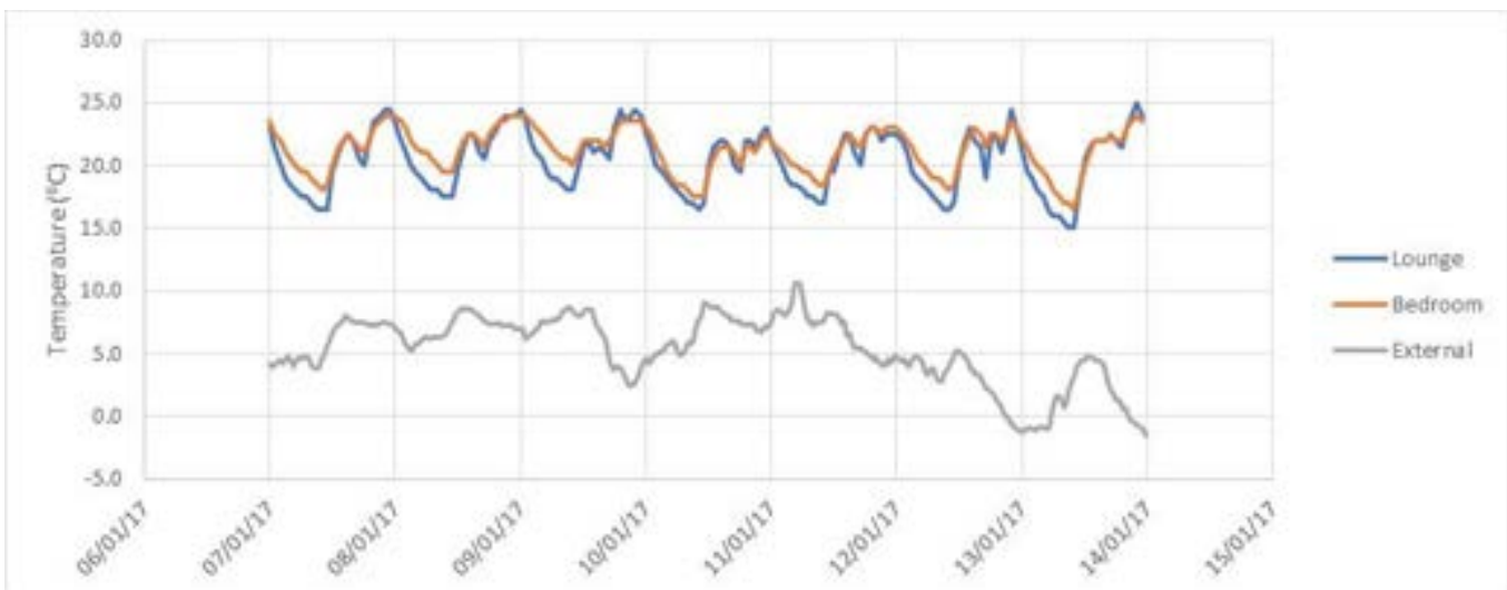
Graph 3.3.11 Property T-20 internal and external temperatures 7 to 14 Jan 2017
