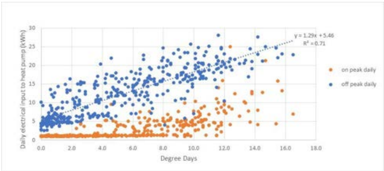
Graph 3.3.30 Property T-9 daily electrical input to heat pump against degree days – 28 Oct 2016 to 4 Dec 2017
