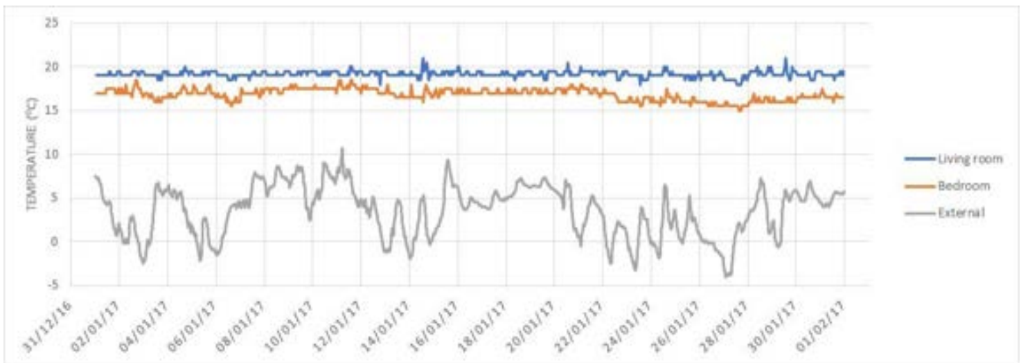
Graph 3.3.3 Property T-10 internal and external temperatures 1 Jan to 31 Jan 2016
