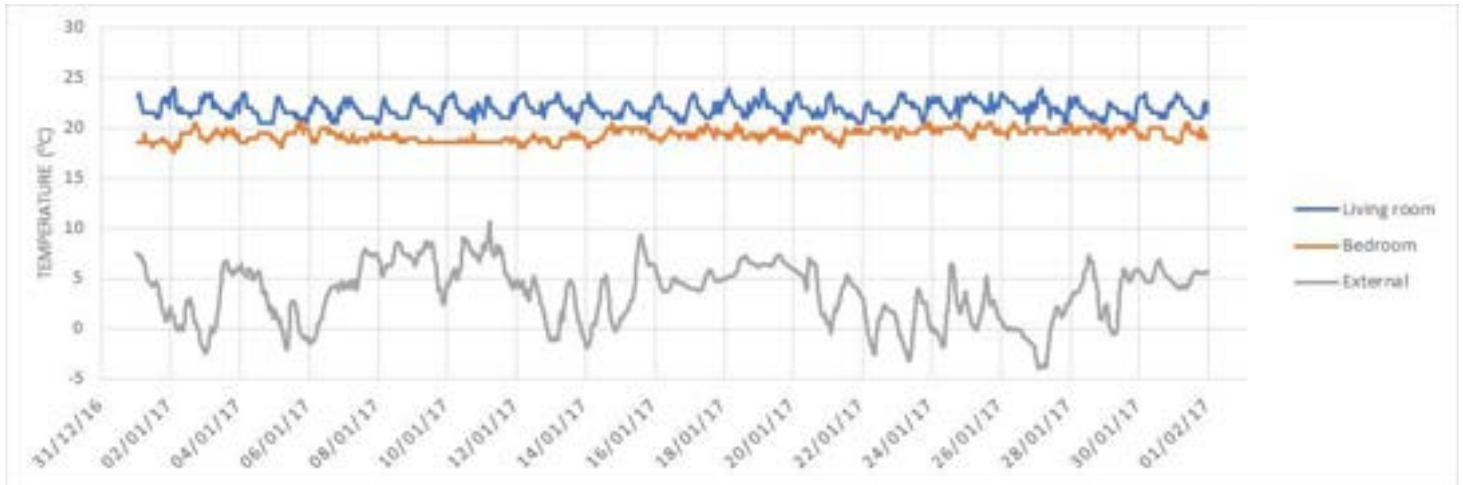
Graph 3.3.4 Property T-22 internal and external temperatures 1 Jan to 31 Jan 2016
