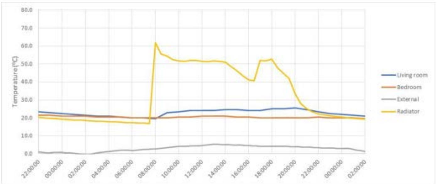
Graph 3.3.39 Property T-13 internal, external and radiator temperatures for 21 Jan 2017
