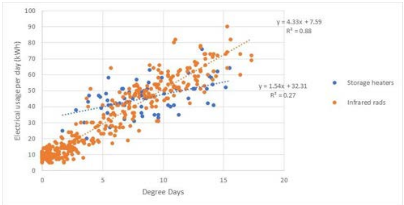
Graph 3.3.9 Property T-22 total daily electrical usage against degree days for 19 Nov 2015 to 10 April 2018
