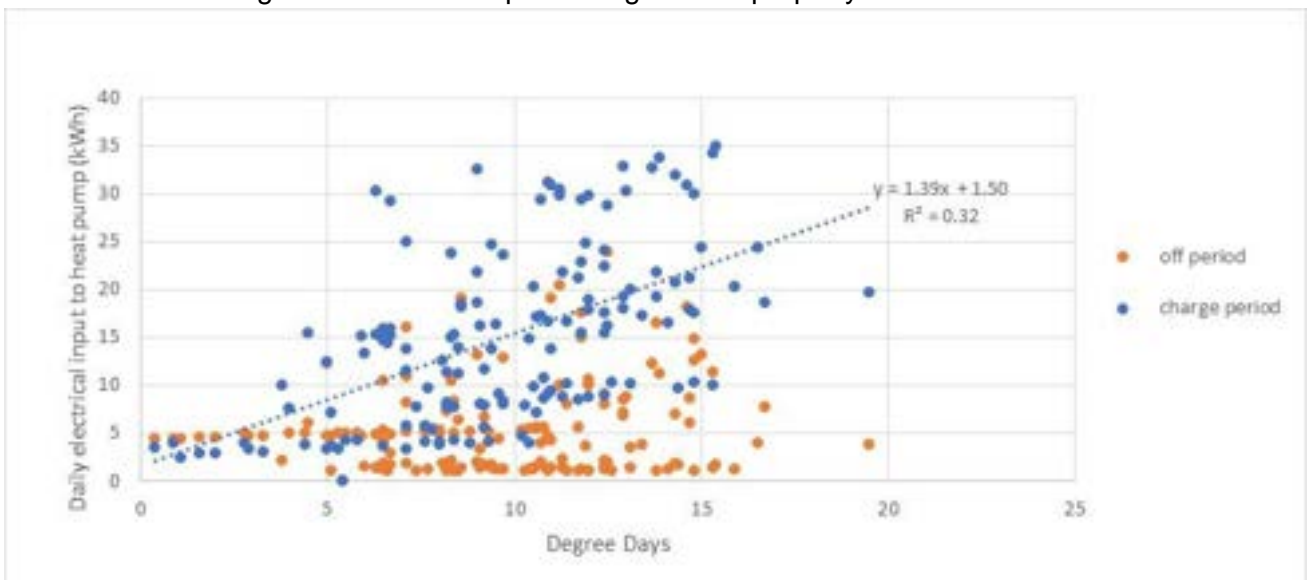
Graph 3.3.31 Property T-13 daily electrical input to heat pump against degree days - 7 Dec 2017 to 1 May 2018
