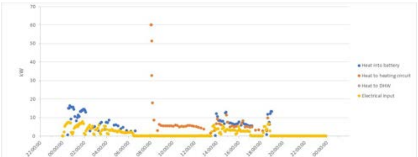
Graph 3.3.37 Property T-9 electrical input and heat output for 26 Jan 2017
