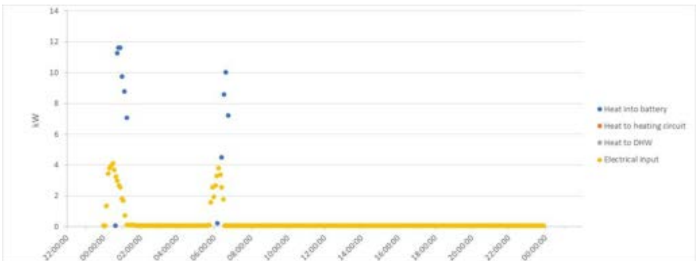
Graph 3.3.40 Property T-9 electrical input and heat output for 15 Jun 2017
