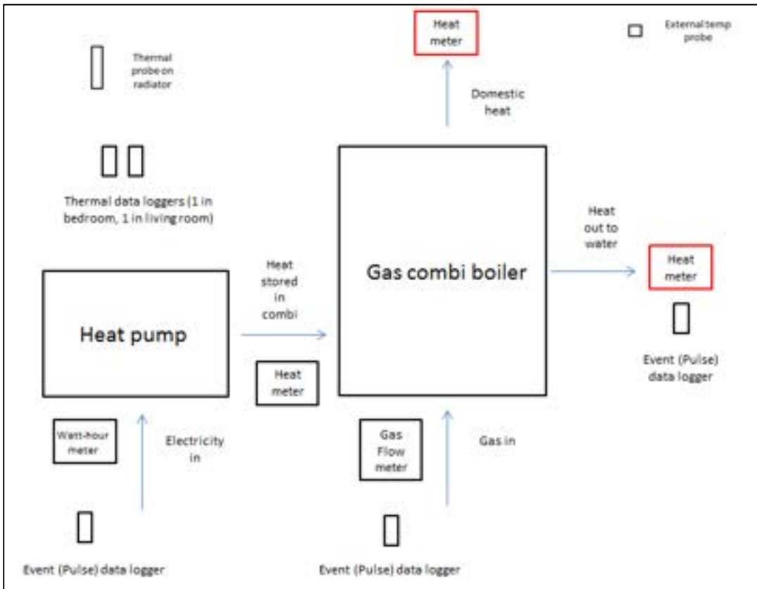
Figure 3.10 – Schematic diagram of monitoring equipment placed in properties receiving hybrid heat pumps,
