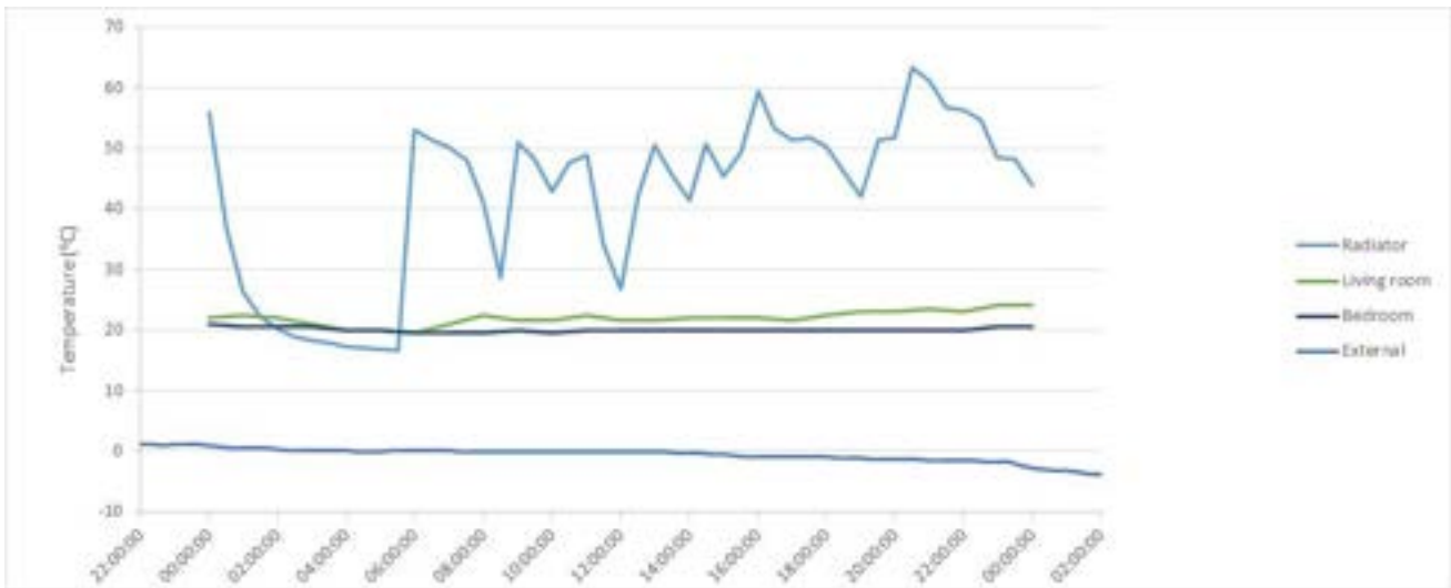
Graph 3.3.34 Property T-8 internal, external and radiator temperatures for 26 Jan 2017
