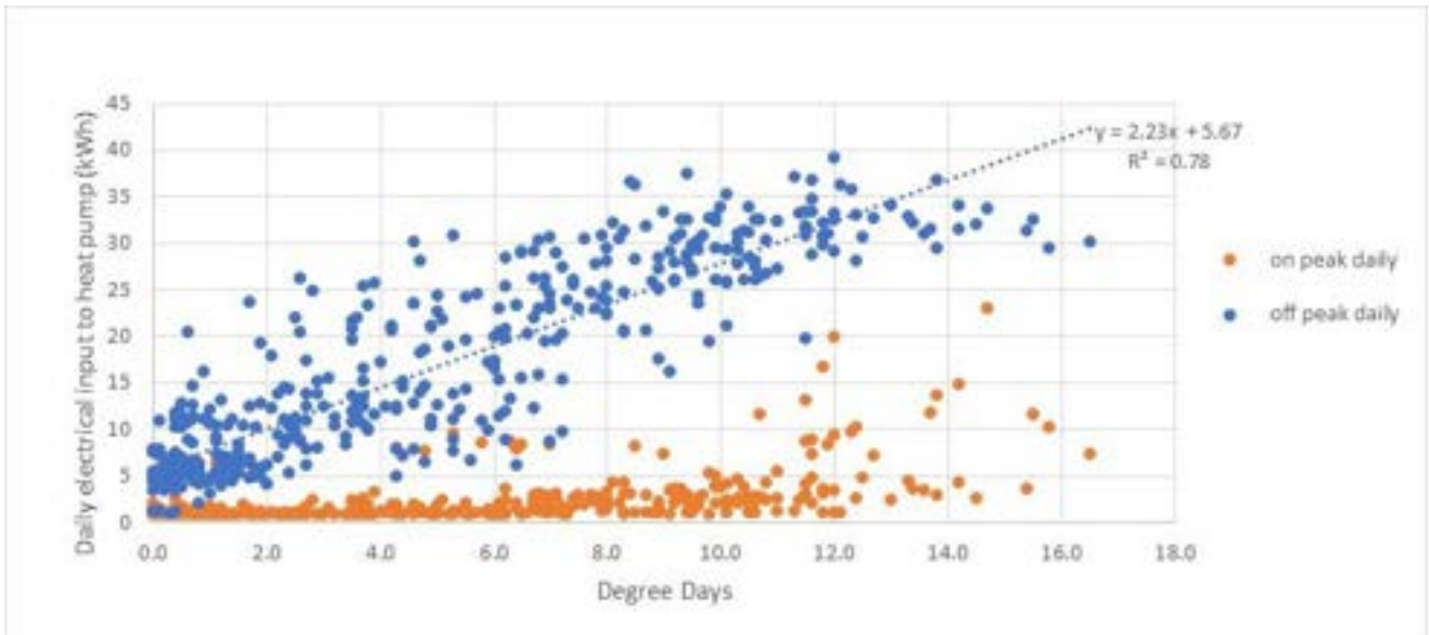
Graph 3.3.27 Property T-8 daily electrical input to heat pump against degree days - 28 Oct 2016 to 6 Dec 2017
