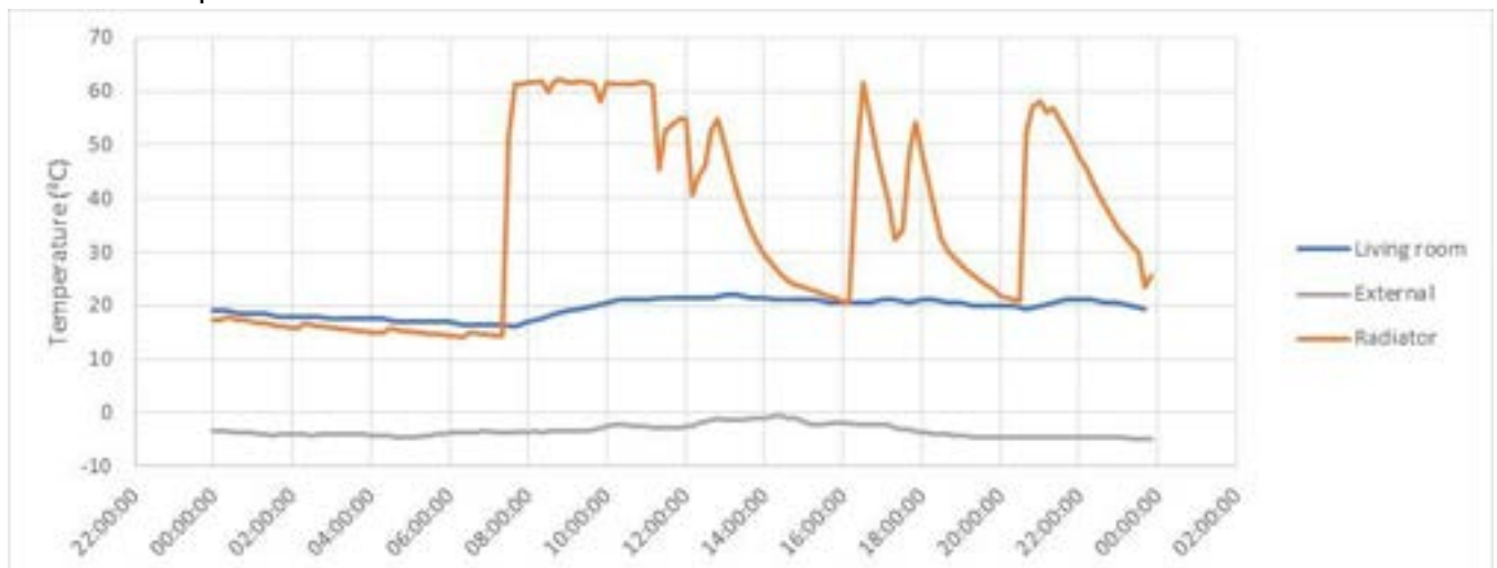
Graph 3.3.14 Property T-73 internal, external and radiator temperatures for 28 Feb 2018
