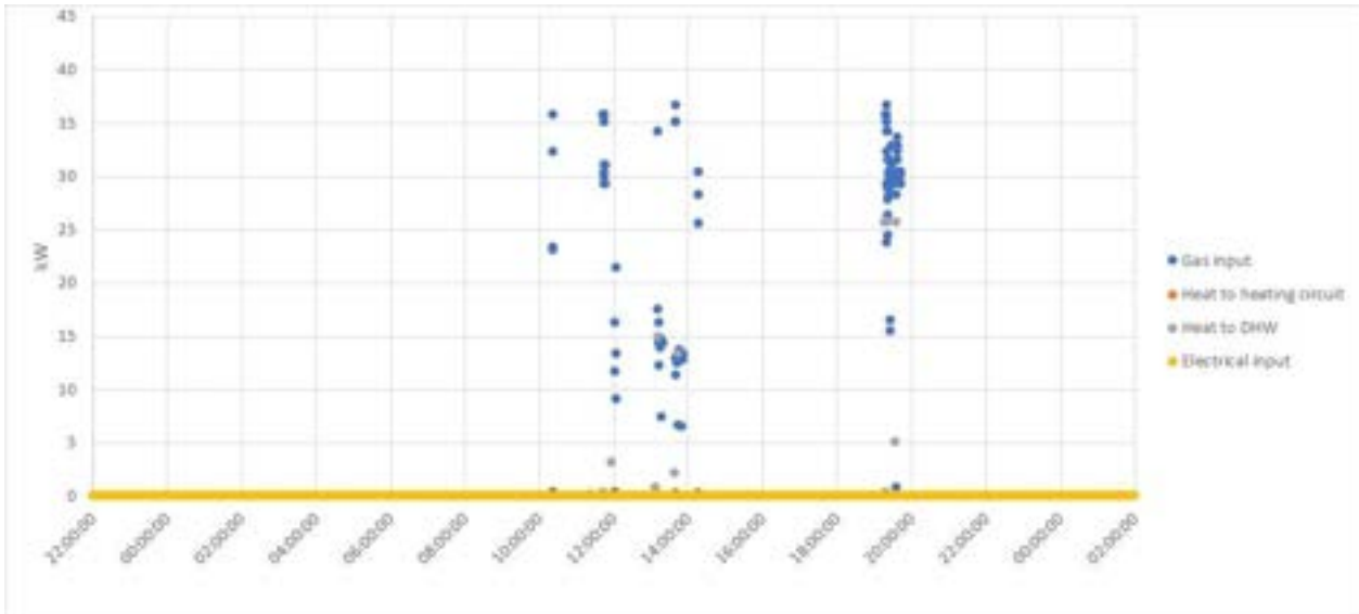
Graph 3.3.17 Property T-73 gas and electrical input to hybrid and heat output for 28 Jan 2018
