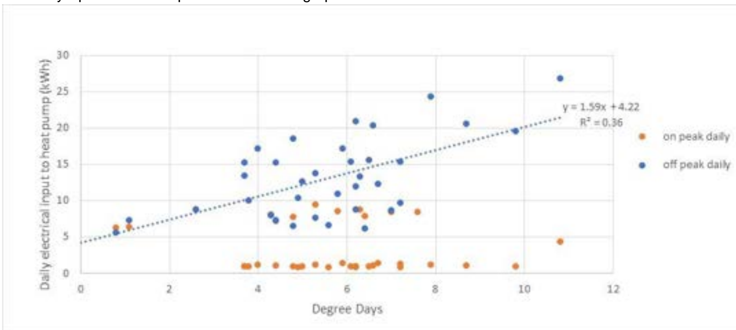
Graph 3.3.28 Property T-8 daily electrical input to heat pump against degree days – 26 Mar to 30 Apr 2017
