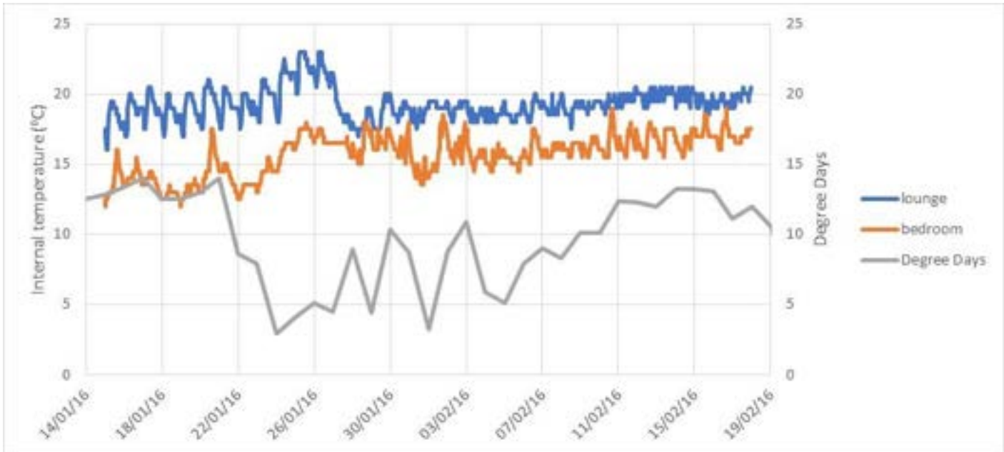
Graph 3.3.2 Property T-5 internal temperatures and degree days 15 Jan to 15 Feb 2016
