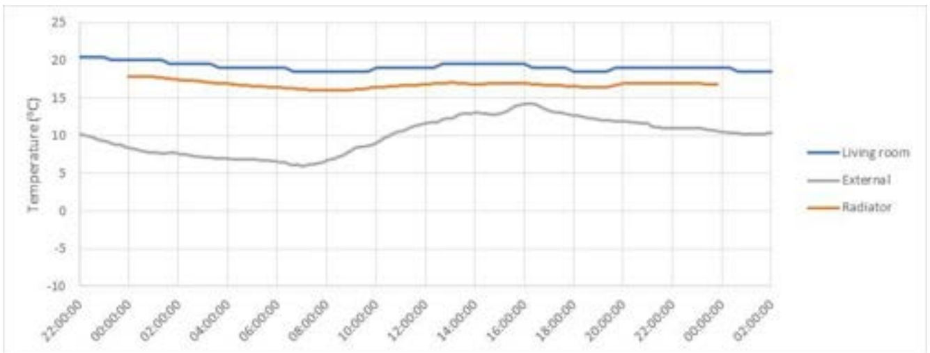
Graph 3.3.18 Property T-73 internal, external and radiator temperatures for 28 Jan 2018
