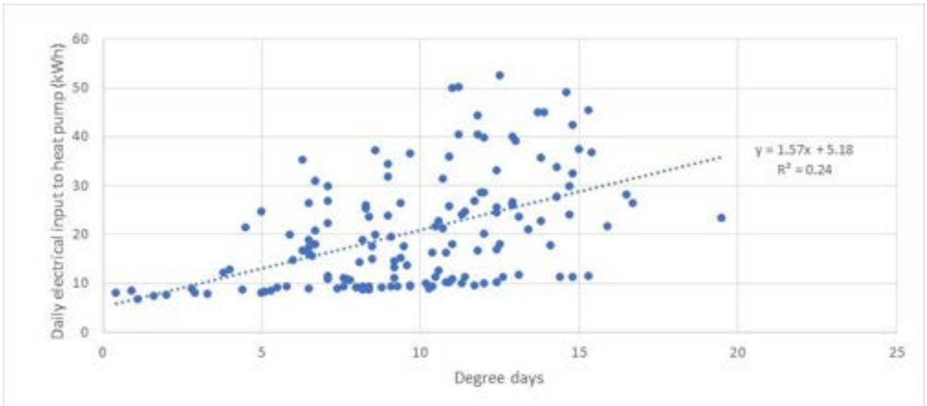
Graph 3.3.32 Property T-13 total daily electrical input to heat pump against degree days - 7 Dec 2017 to 1 May 2018
