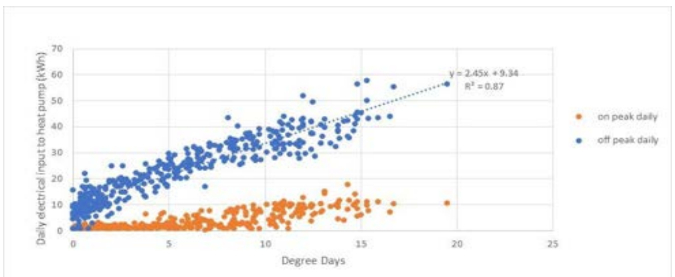
Graph 3.3.26 Property T-23 daily electrical input to heat pump against degree days – 8 Apr 2017 to 28 Apr 2018
