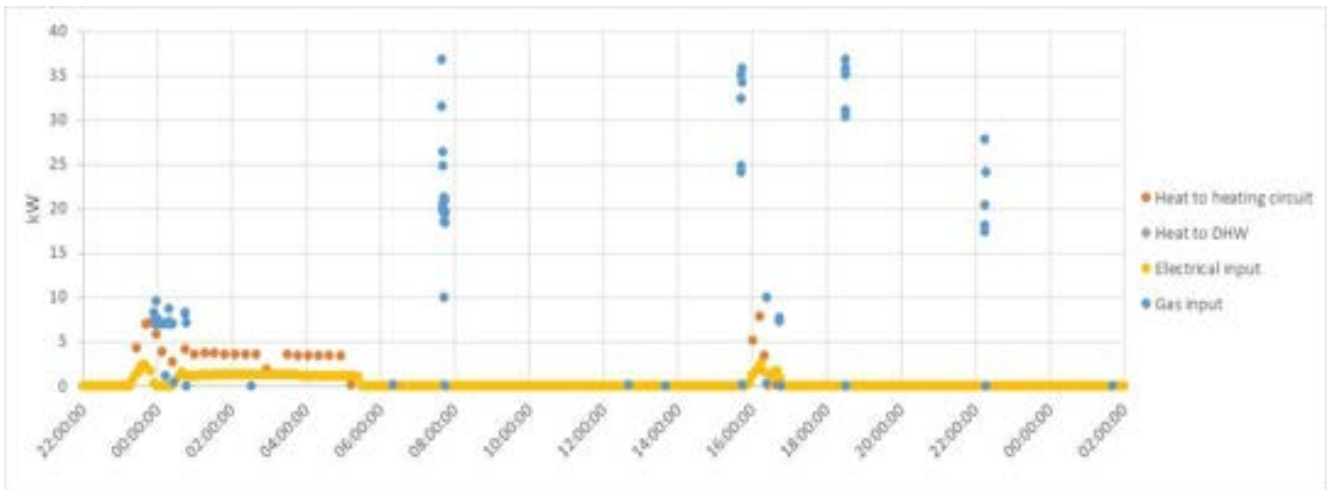
Graph 3.3.19 Property T-83 gas and electrical input to hybrid and heat output for 4 Jan 2018
