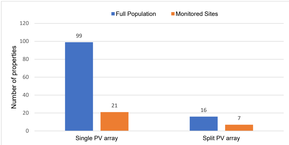
Figure 2.4 Number of properties with single or split solar PV arrays
