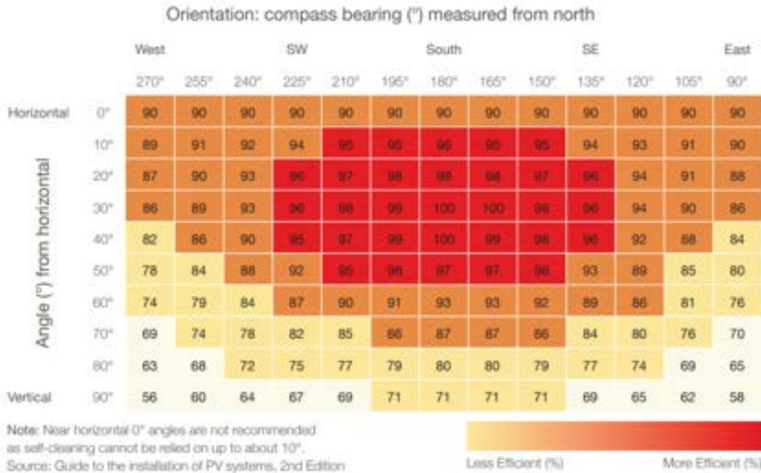
Figure 1.4 Percentage of the maximum possible yield from a solar PV system in the UK for different orientations and inclinations (Graphic from Mitsubishi Electric Information Guide, Photovoltaic Systems, Issue 40)
