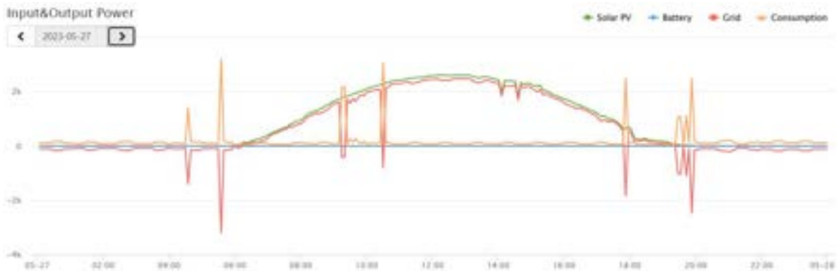
Figure 4.6 Input & Output Power graph for household WS-05 on 27 May 23
