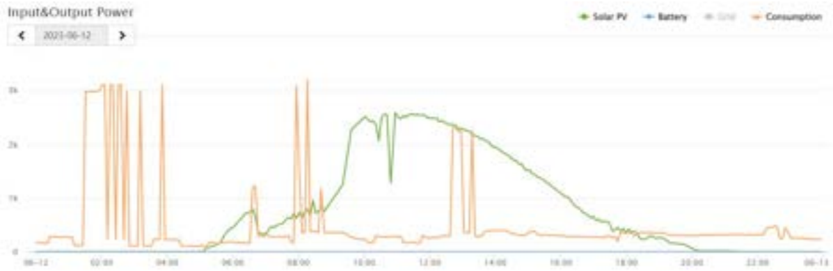
Figure 4.8 Input & Output Power graph for household WS-06 on 12 Jun 23
