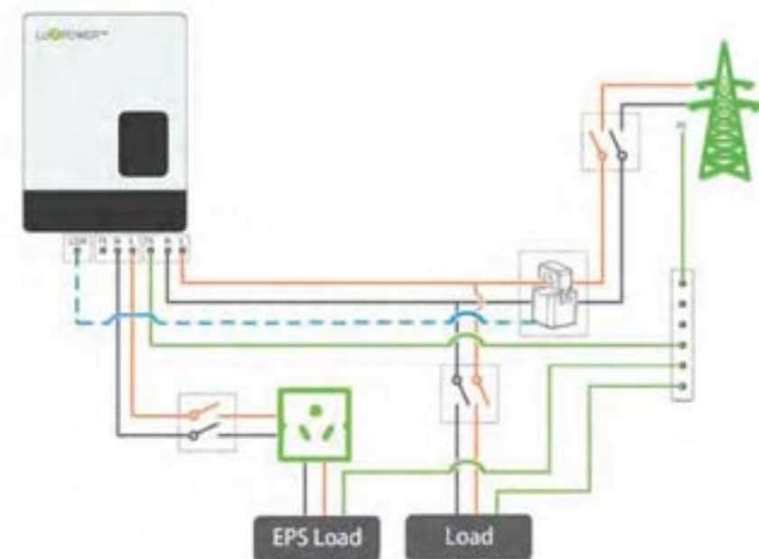
Figure 3.2 Wiring diagram for the LuxPower LXP3600 hybrid inverter with a CT clamp 9
