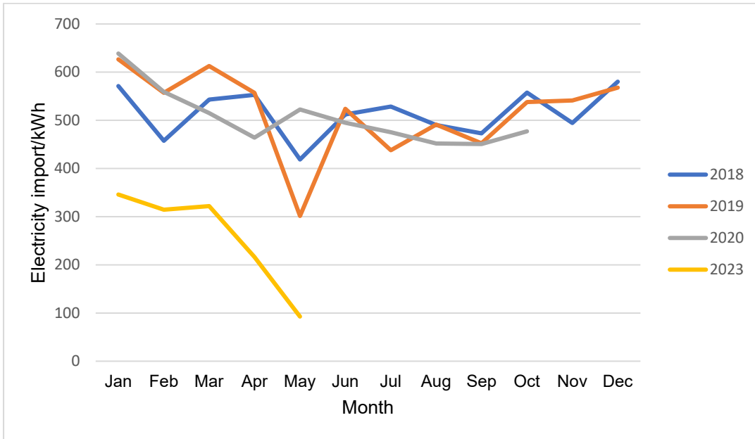
Figure 4.14 Graph of electricity import per month for household WS-13 from smart meter data
