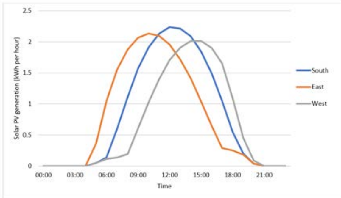
Figure 1.5 Illustration of how solar PV generation can vary on a sunny day for different orientated solar PV arrays
