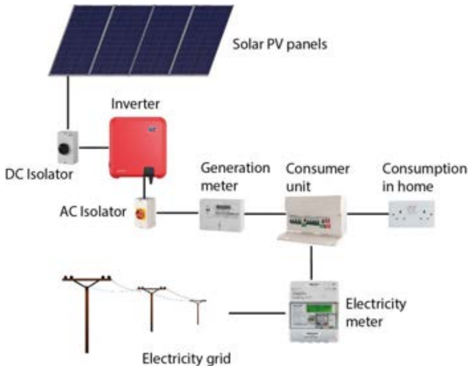
Figure 1.3 Schematic diagram of components in a domestic solar PV system
