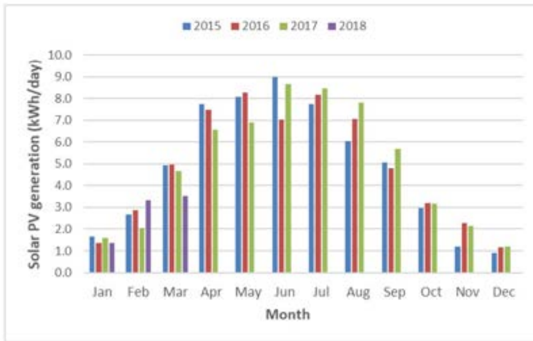
Figure 1.6 Variation in solar PV generation between 2015 and 2018 for a 2.35kW solar PV system in London orientated 60 degrees from south
