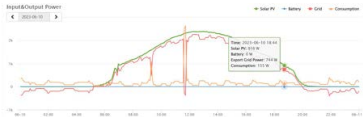
Figure 3.5 Input & Output Power graph for a household on 10 Jun 2023
